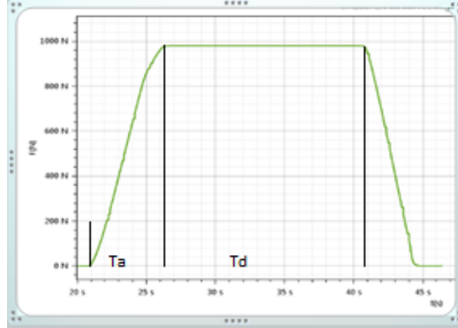
Measurement Cycle for Brinell Hardness Scales
