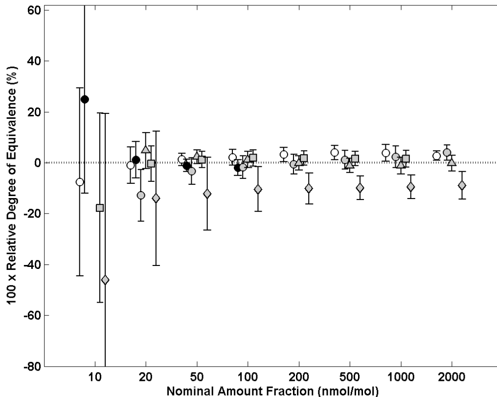
Figure 13 Relative degree of equivalence for each NMI using travelling standard 2 at each amount fraction. Data from NIST, NPL-GMTA, NPL-TH, PTB and NMIJ are represented with \circ , \bullet , \blacklozenge , \blacktriangle and \blacksquare respectively. A second data set collected at NIST after the comparison is represented with \bullet . Bars indicate estimated uncertainties on the generated amount fractions of water by each institute at the 95% confidence interval.
