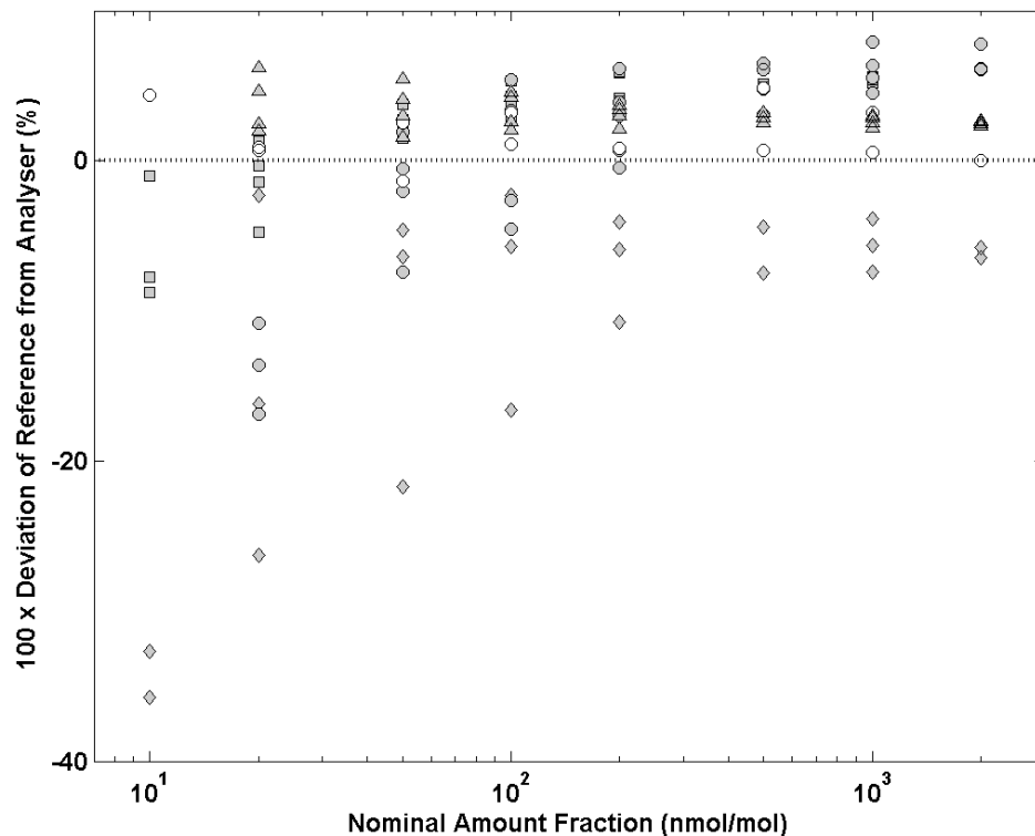
Figure 11 Deviation of the dynamic reference generated at each NMI from travelling standard 2. Data from NIST, NPL-GMTA, NPL-TH, PTB and NMIJ are represented with \circ , \bullet , \blacklozenge , \blacktriangle and \blacksquare respectively.
