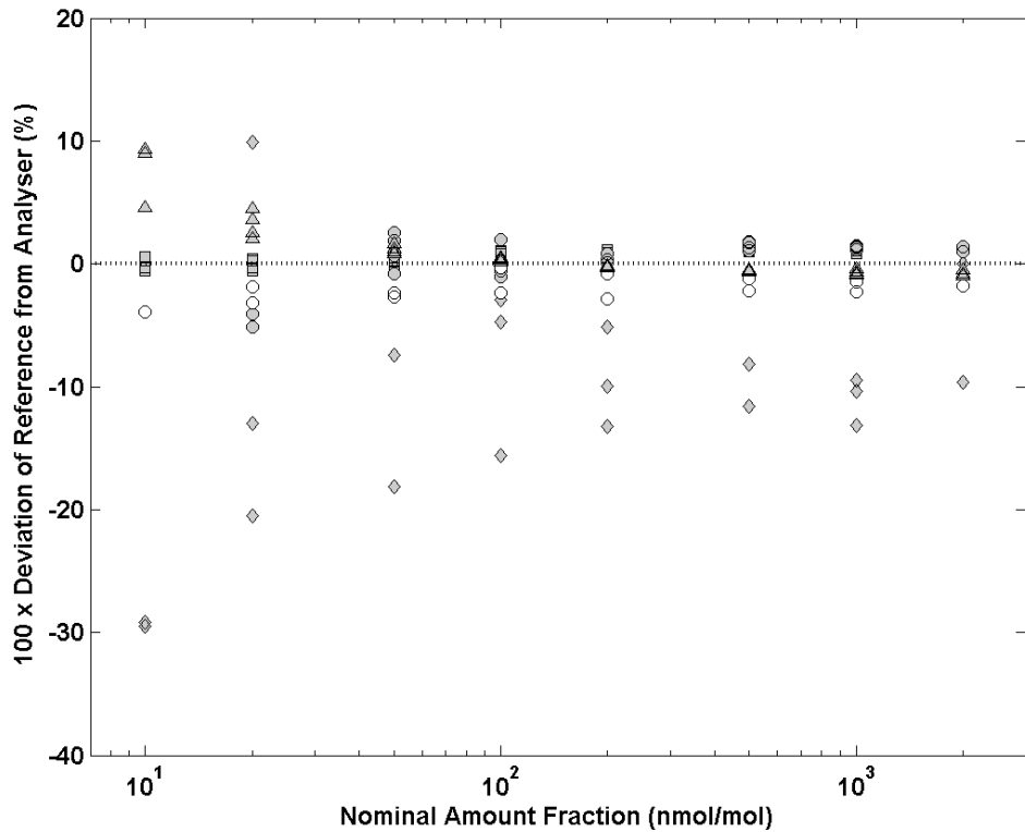
Figure 7 Deviation of the dynamic reference generated at each NMI from travelling standard 1. Data from NIST, NPL-GMTA, NPL-TH, PTB and NMIJ are represented with \circ , \bullet , \blacklozenge , \blacktriangle and \blacksquare respectively.
